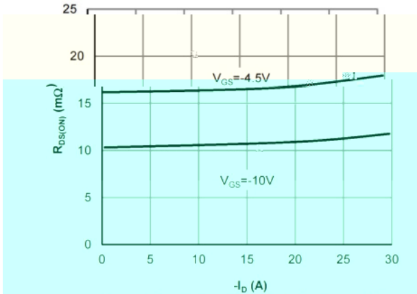
Figure 3: On-Resistance vs. Drain Current and Gate
